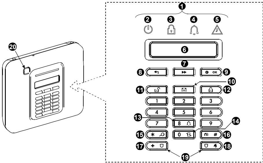
Figure 1a. WP Panel Controls and Indicators
