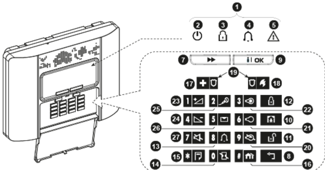
Figure 1b. WP Panel Controls and Indicators
